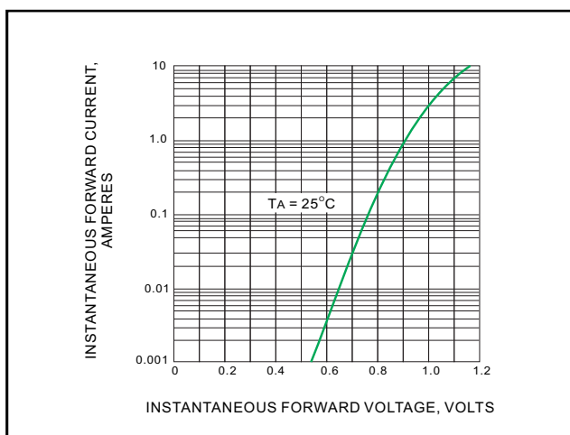
FIG.4TYPICALFORWARDCHARACTERISTICS
