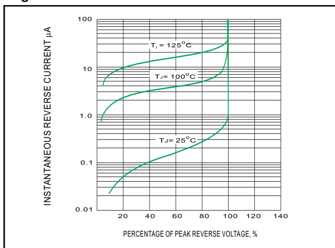
Fig.3-TYPICAL REVERSE CHARACTERISTIC
