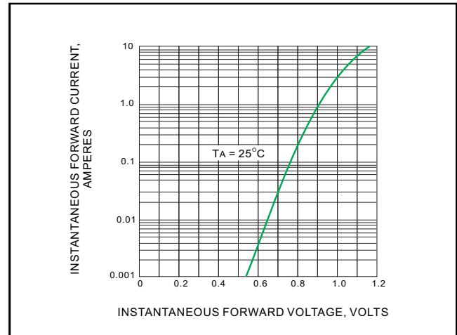
FIG.4TYPICALFORWARDCHARACTERISTICS
