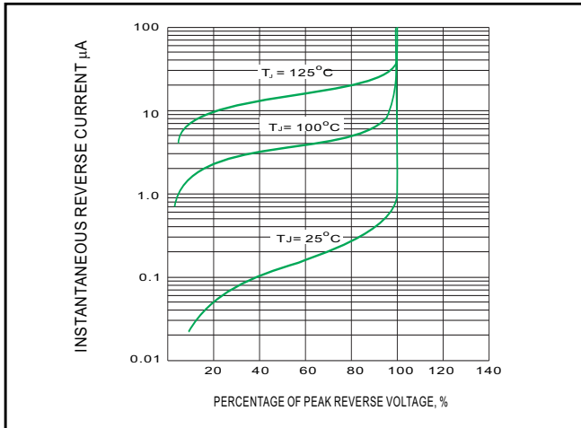
Fig.3-TYPICAL REVERSE CHARACTERISTIC
